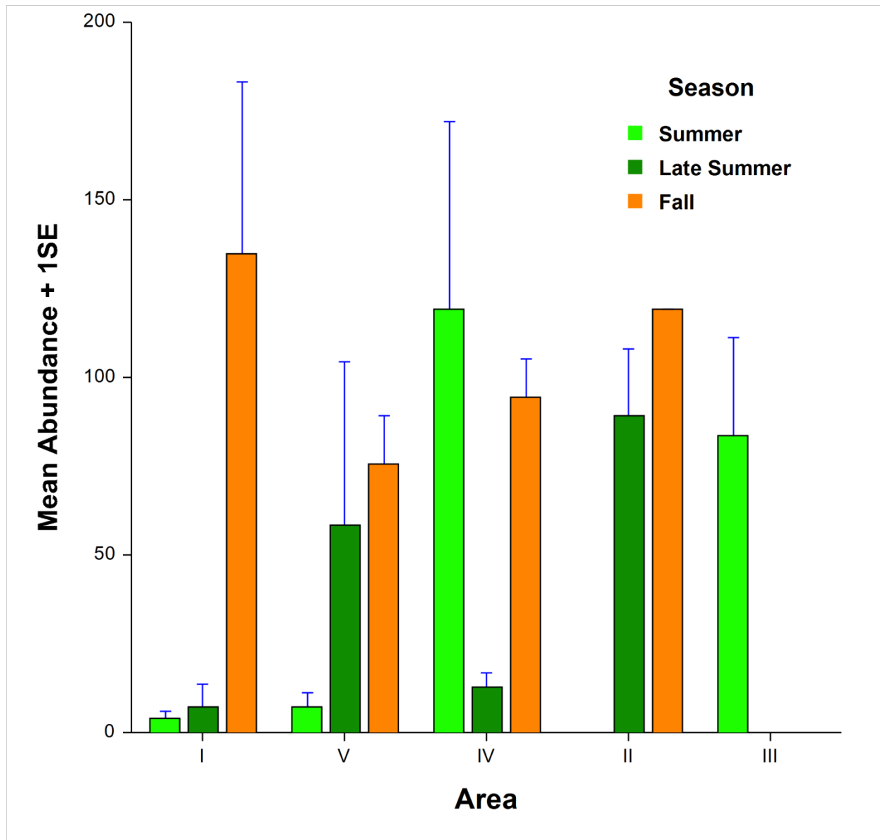
Figure 4. Seasonal differences in benthic community mean abundance ( + 1 standard error, per 20\text{ cm}^2 ) among the different sampling areas in New Haven Harbor. Areas I and V are where extensive accumulations of macroalgae were found in previous studies; Area IV is a transitional area where some accumulations were found; Areas II and III had little to no drift macroalgae.
